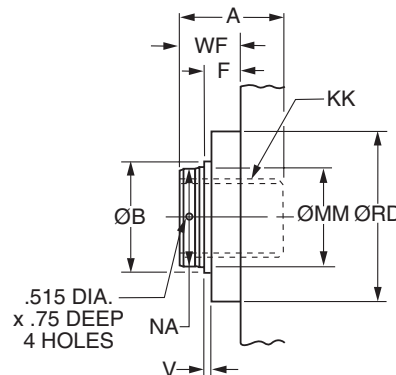
Thread Style 9 2 (NFPA Style SF) Small Female
