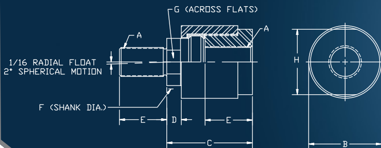
Alignment Coupler 1/16 Radial Float 2°
